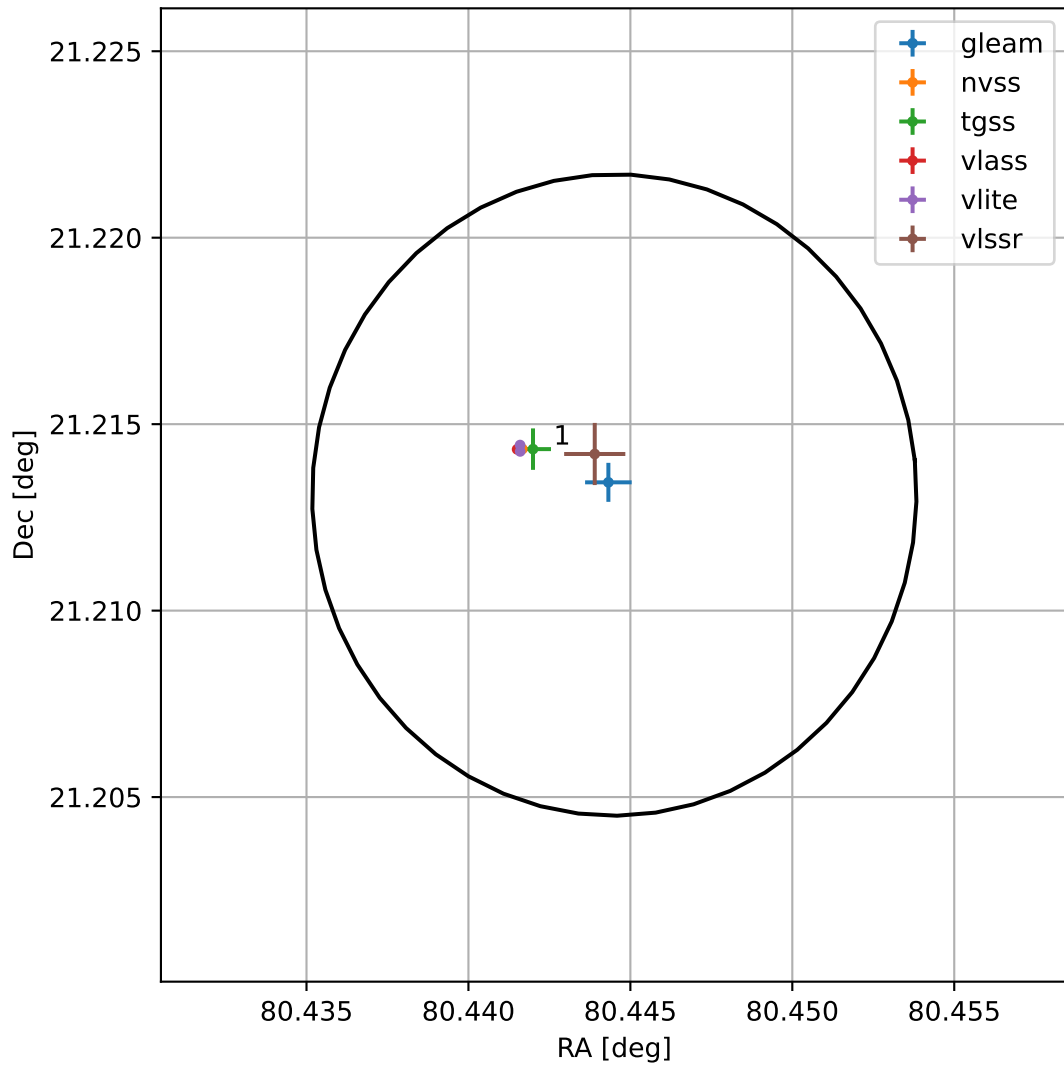
4FGL J0521.7+2112
