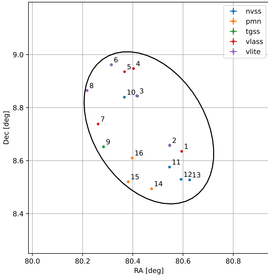
4FGL J0521.8+0843
