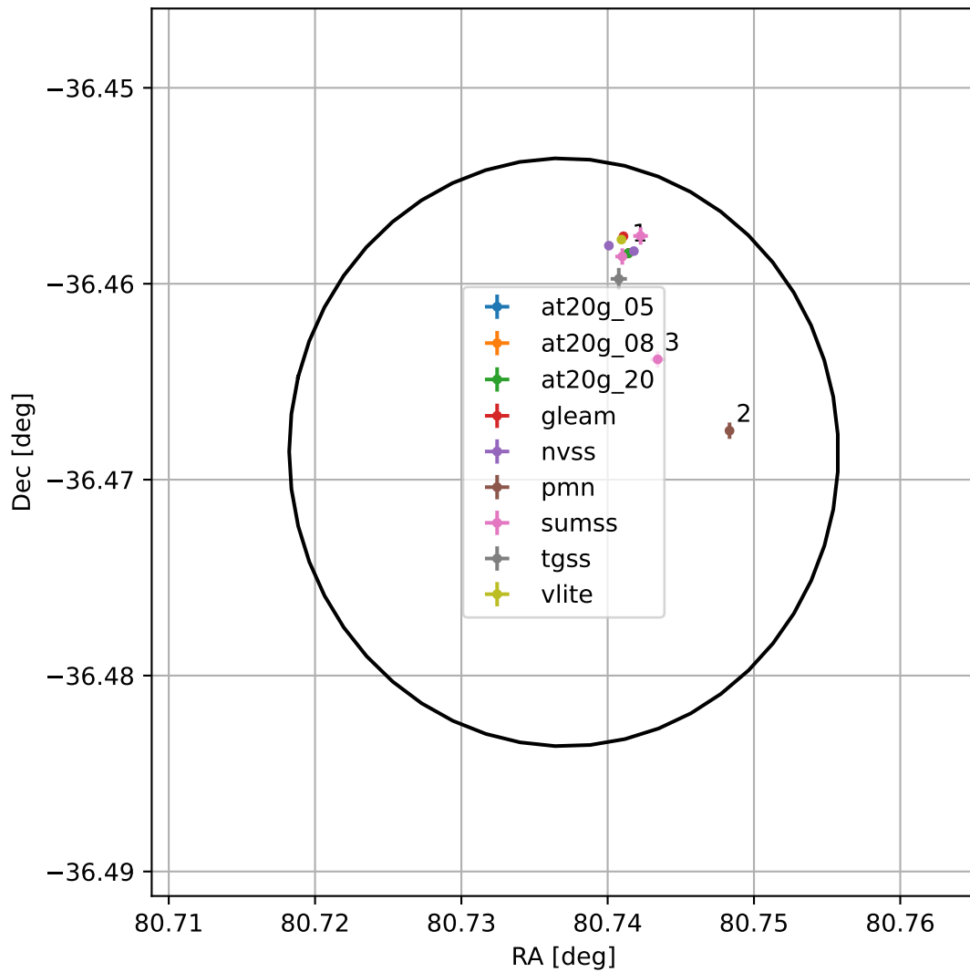
4FGL J0522.9-3628
