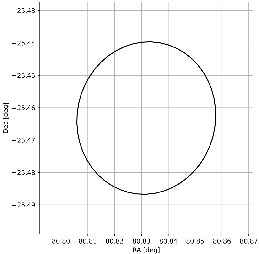
4FGL J0523.3-2527
