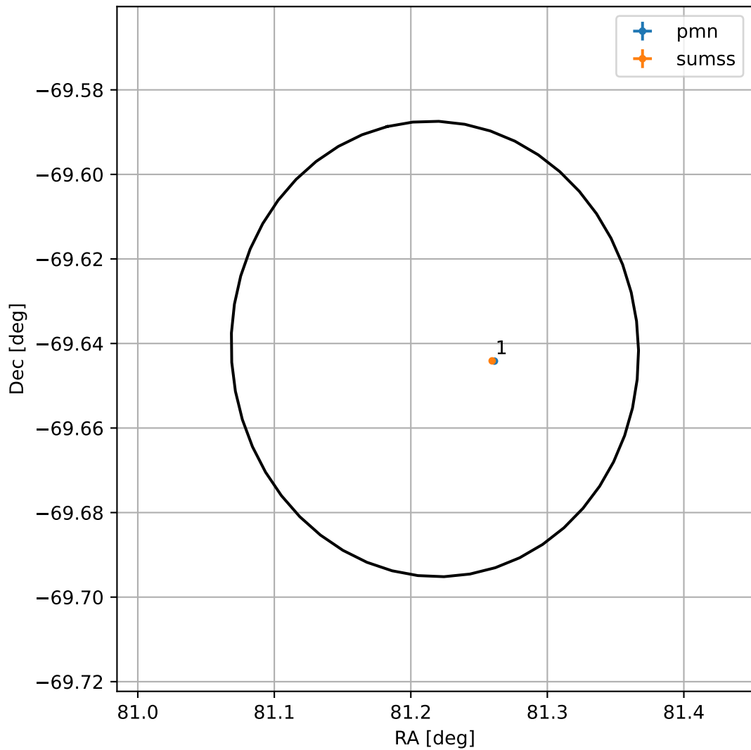
4FGL J0524.8-6938
