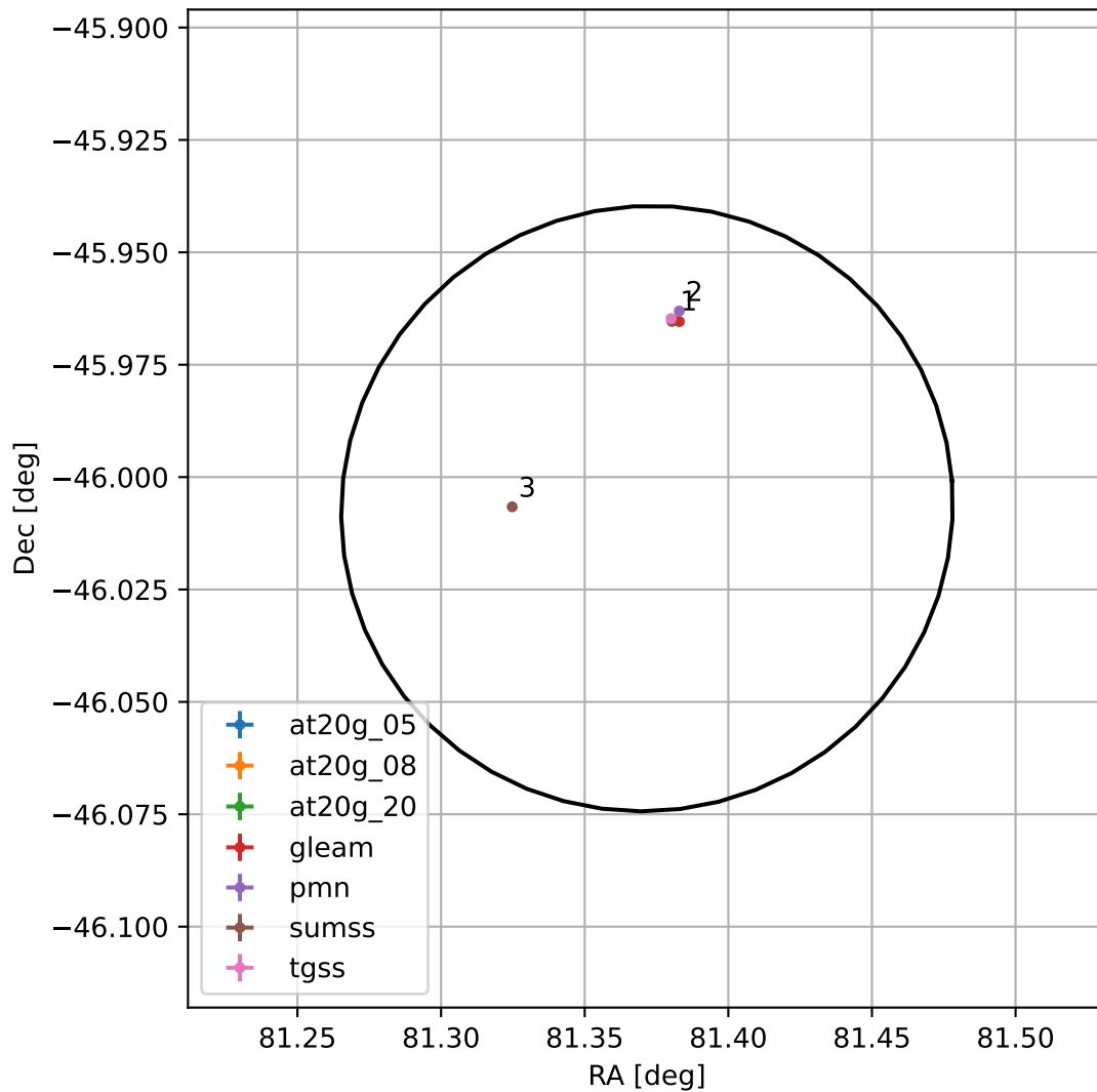
4FGL J0525.4-4600
