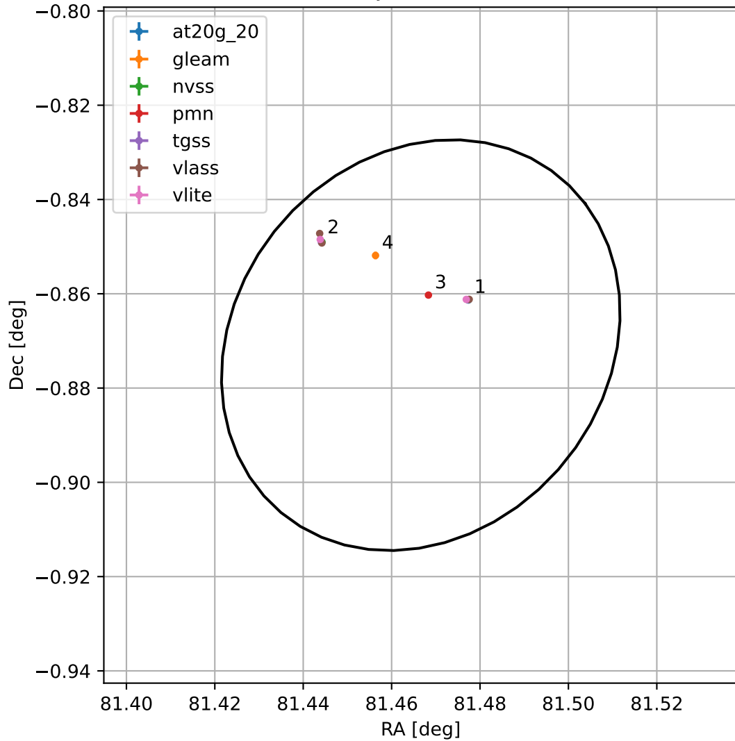
4FGL J0525.8-0052
