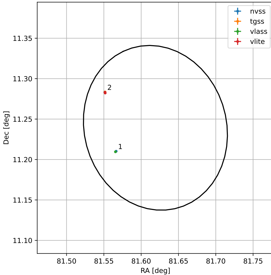
4FGL J0526.4+1114
