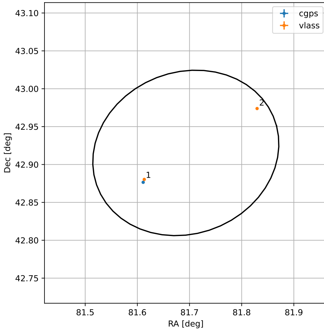
4FGL J0526.7+4254
