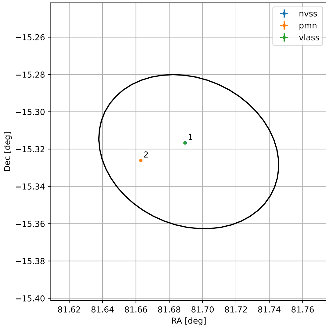
4FGL J0526.7-1519
