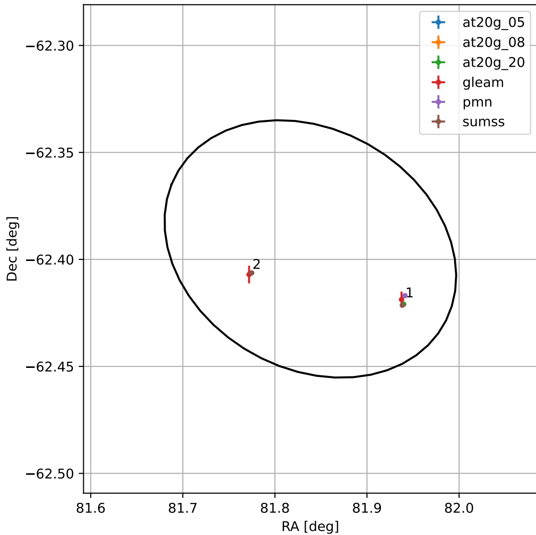
4FGL J0527.3-6223
