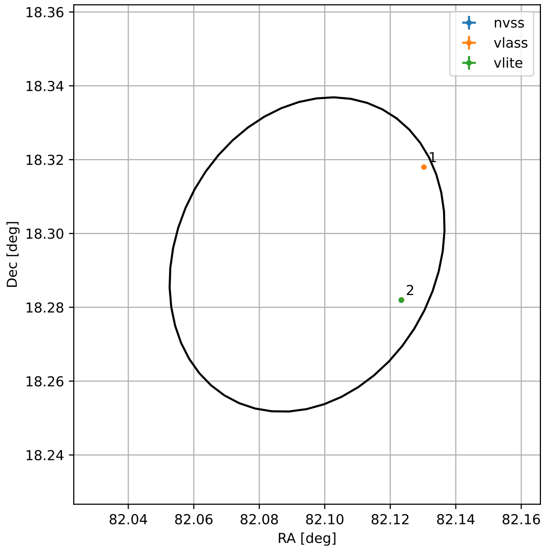
4FGL J0528.3+1817
