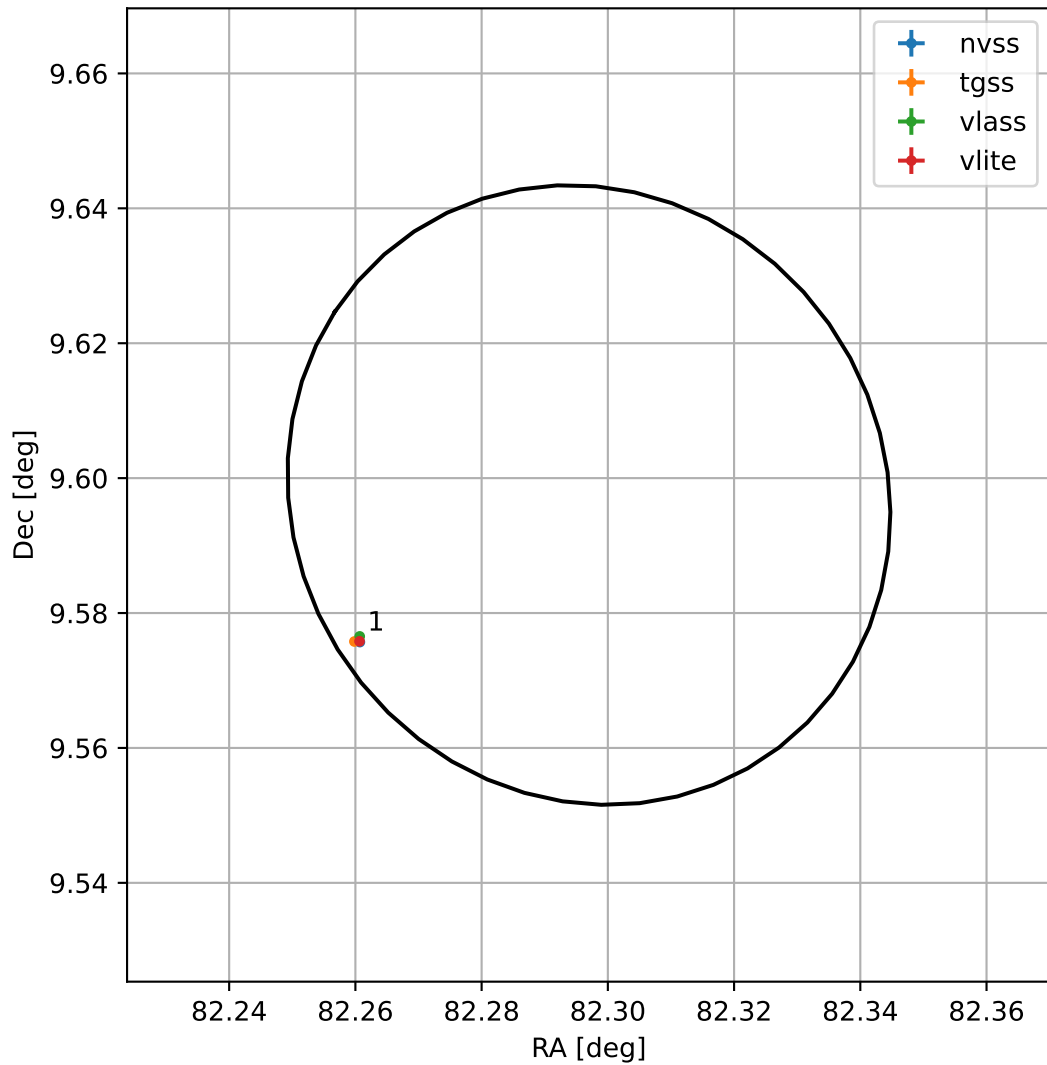
4FGL J0529.1+0935
