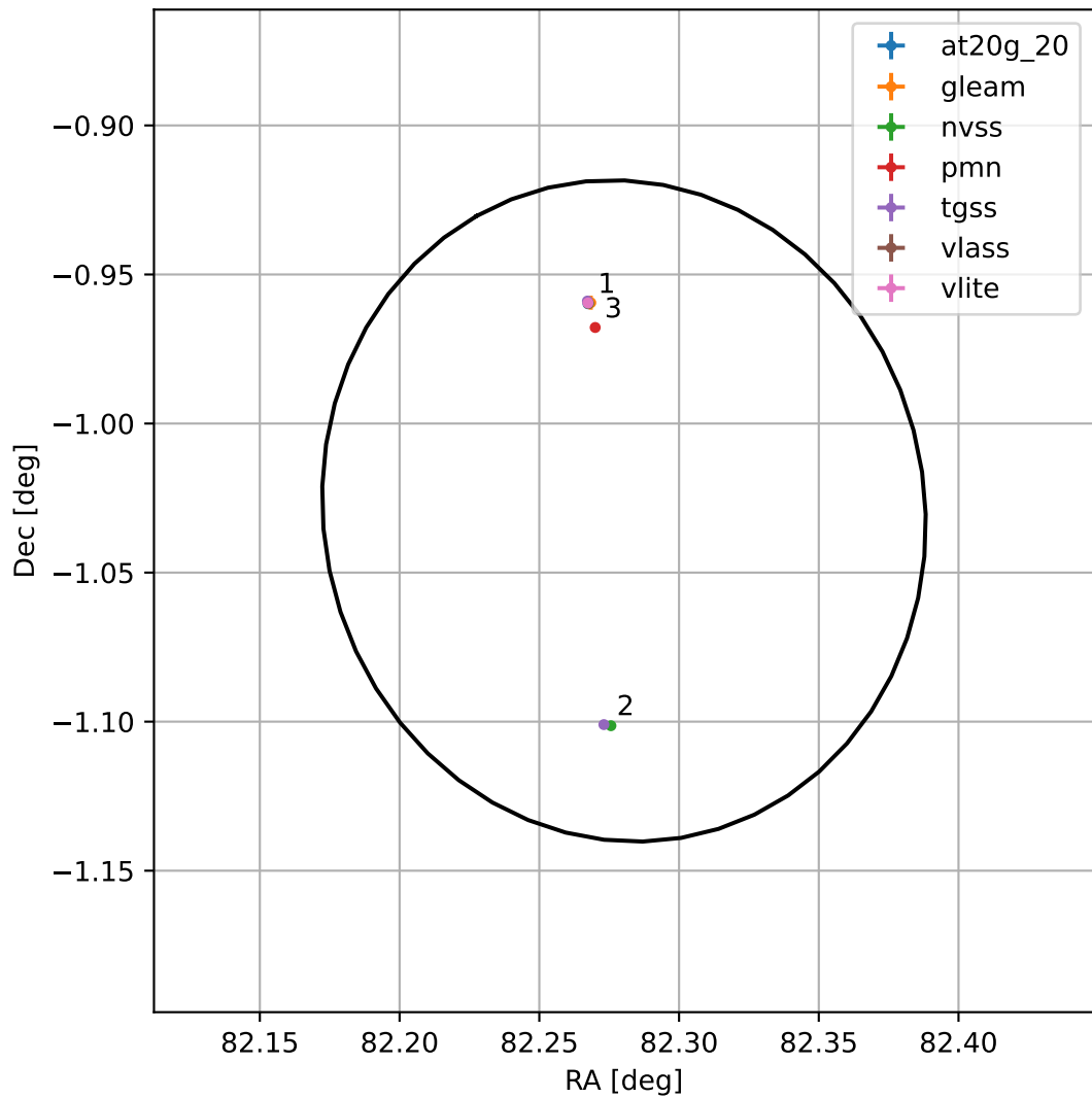
4FGL J0529.1-0101
