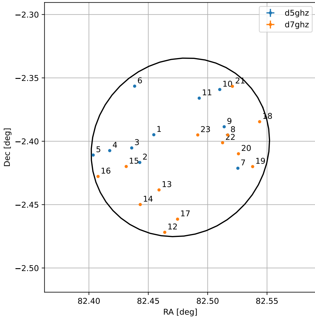
4FGL J0529.9-0224
