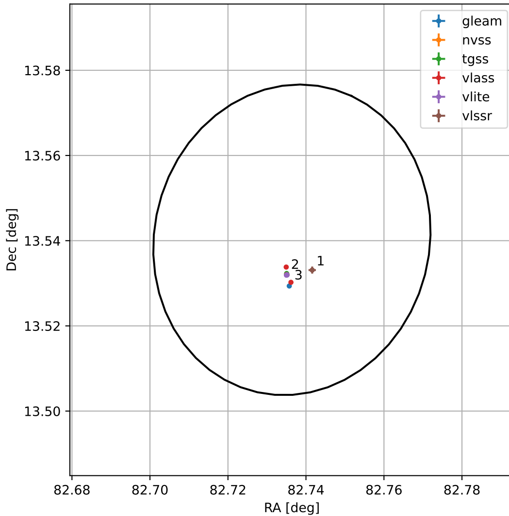
4FGL J0530.9+1332
