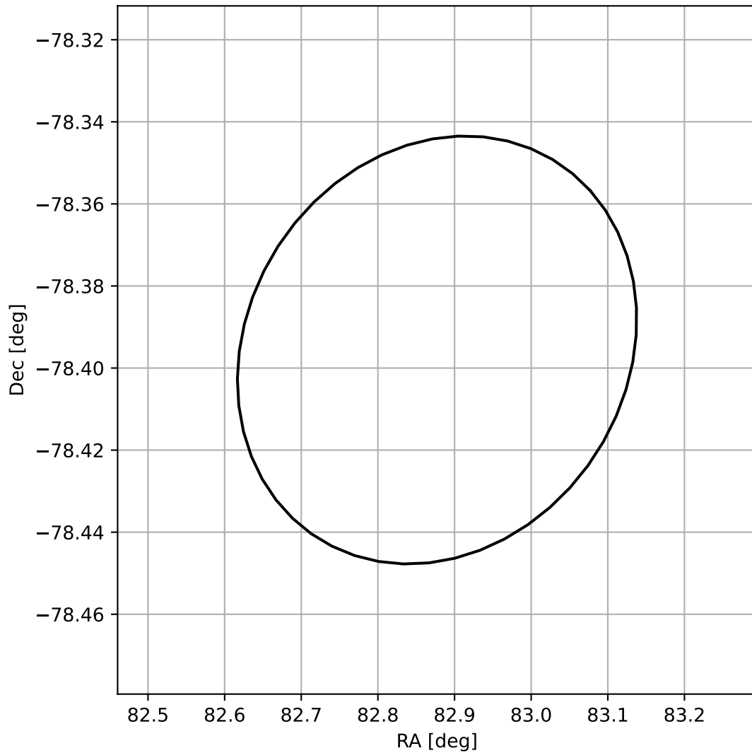
4FGL J0531.5-7823
