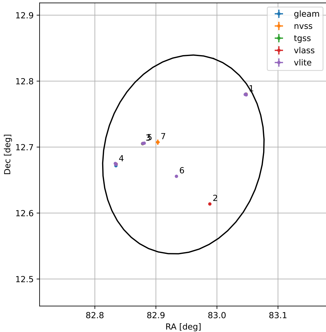
4FGL J0531.7+1241
