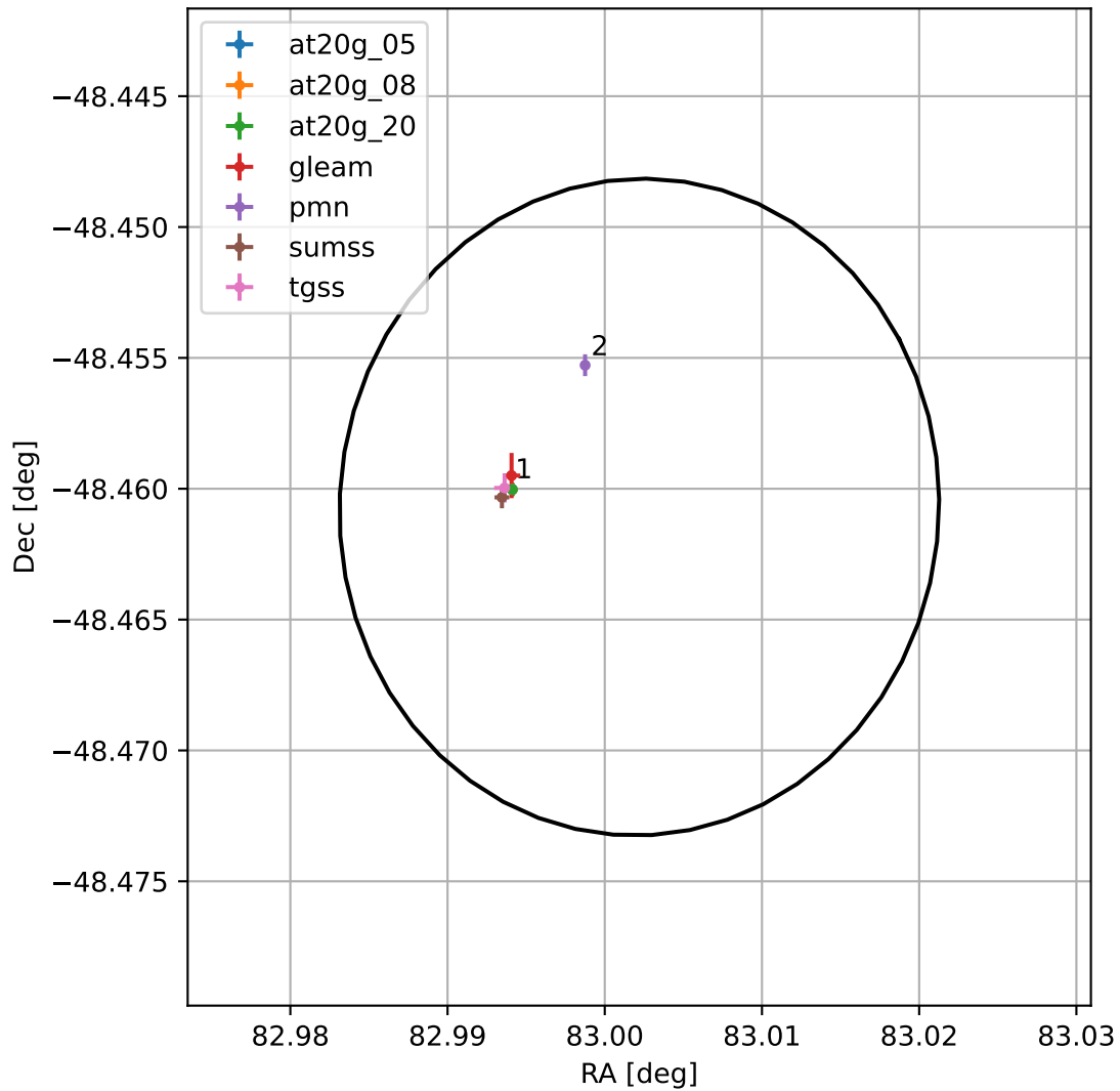
4FGL J0532.0-4827
