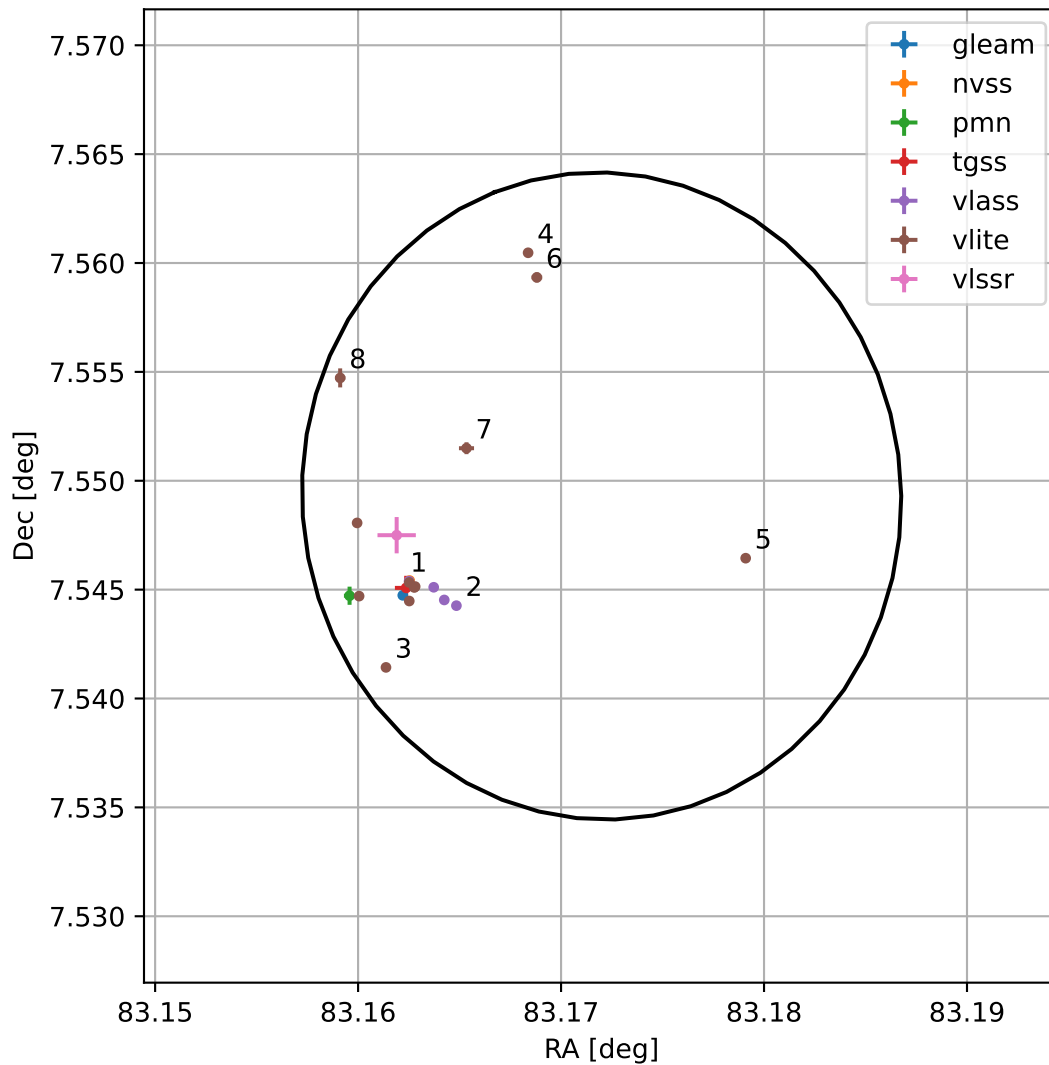
4FGL J0532.6+0732
