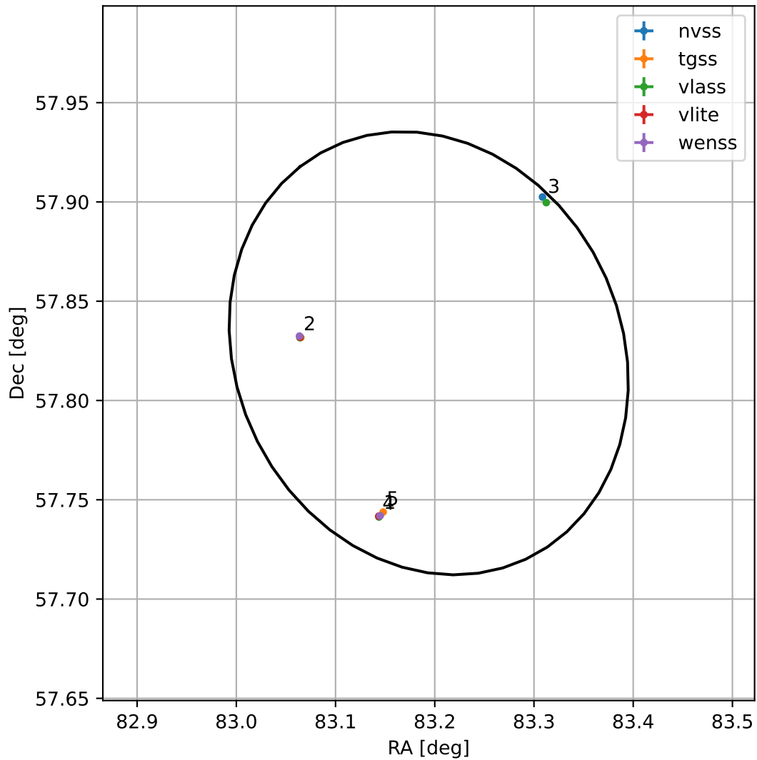
4FGL J0532.7+5749
