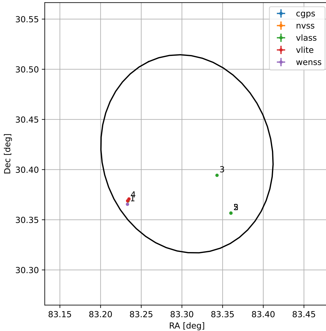
4FGL J0533.2+3024
