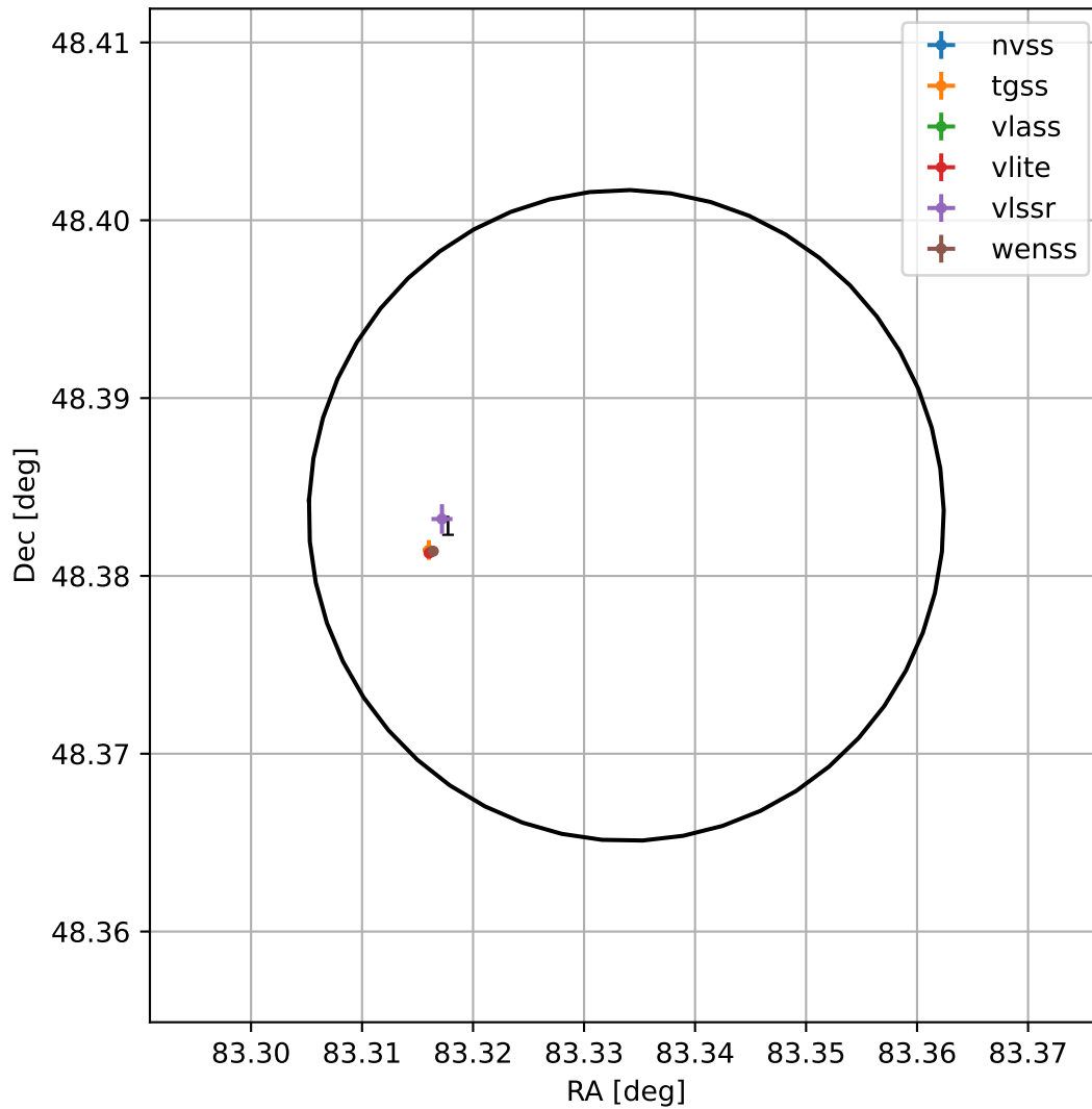
4FGL J0533.3+4823
