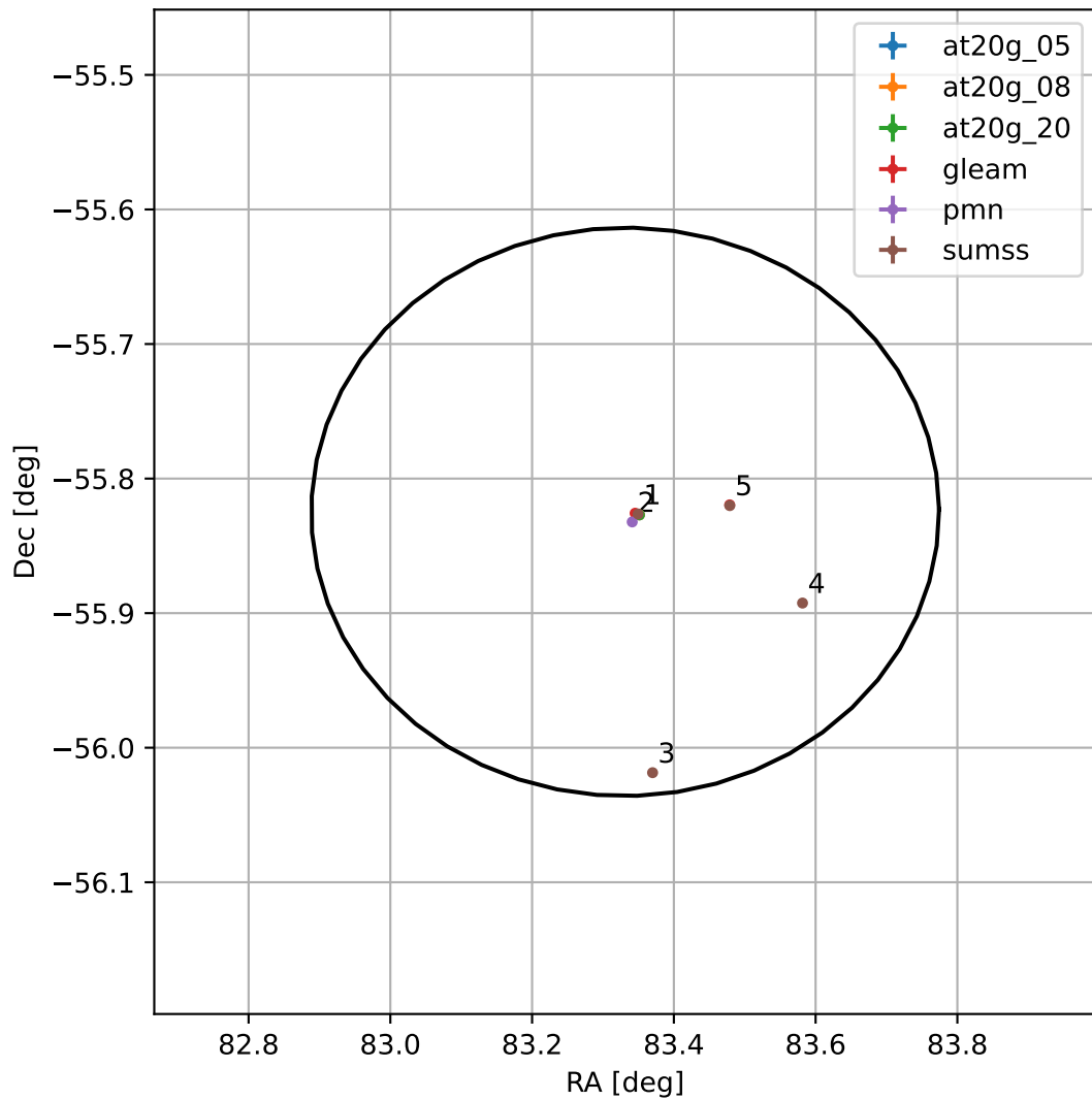
4FGL J0533.3-5549
