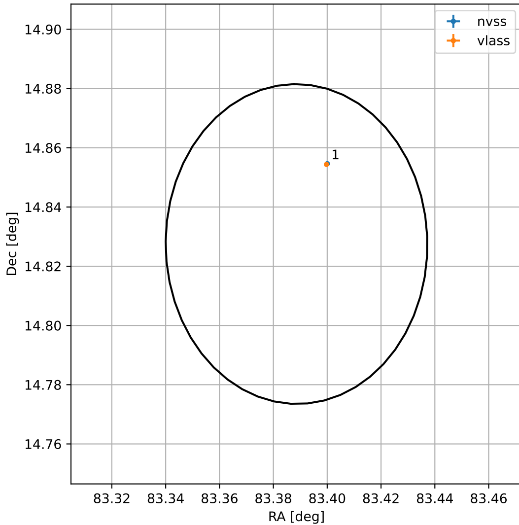
4FGL J0533.5+1449
