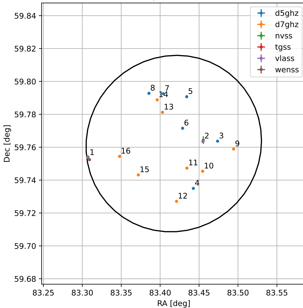
4FGL J0533.6+5945
