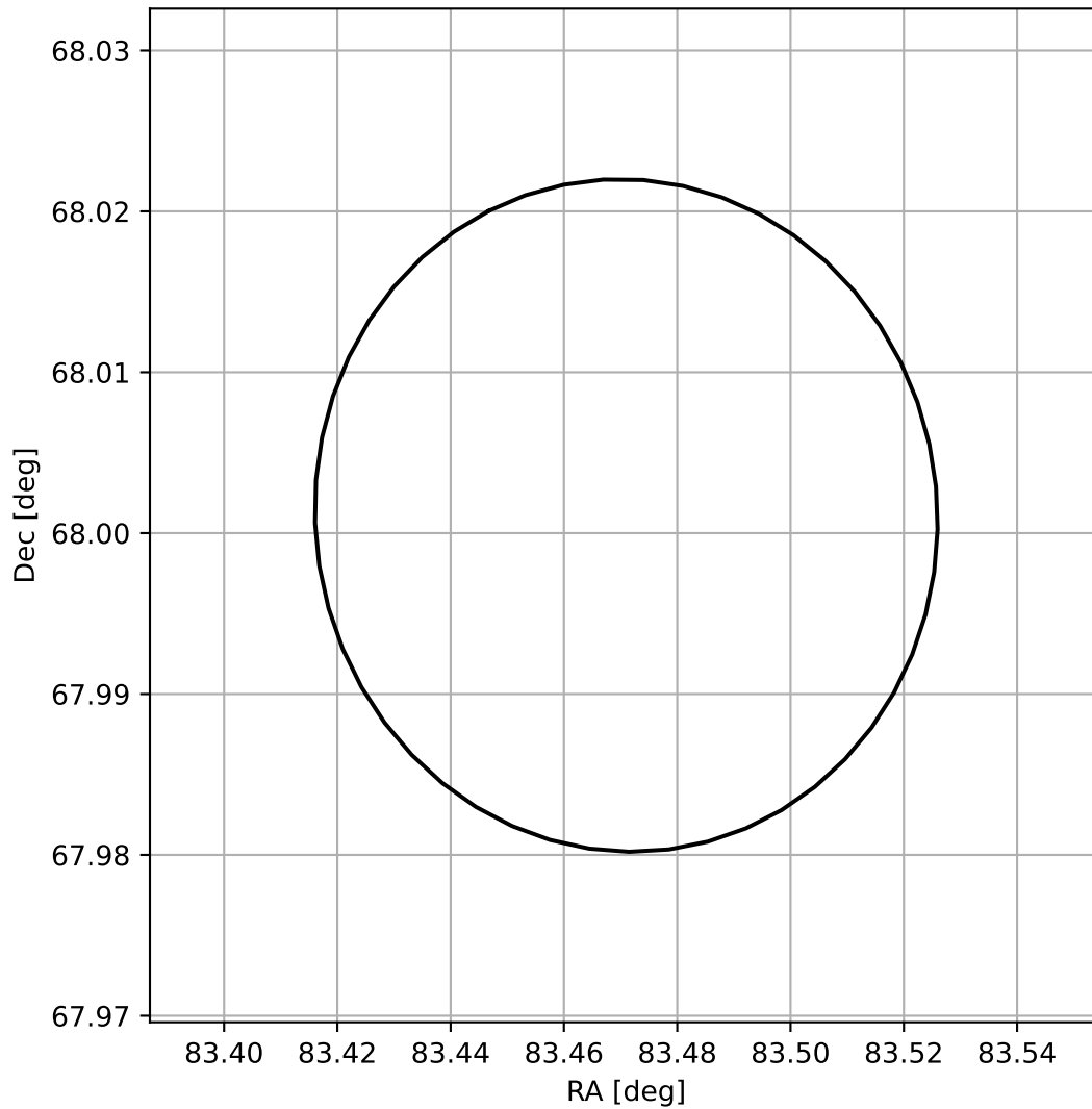
4FGL J0533.8+6800
