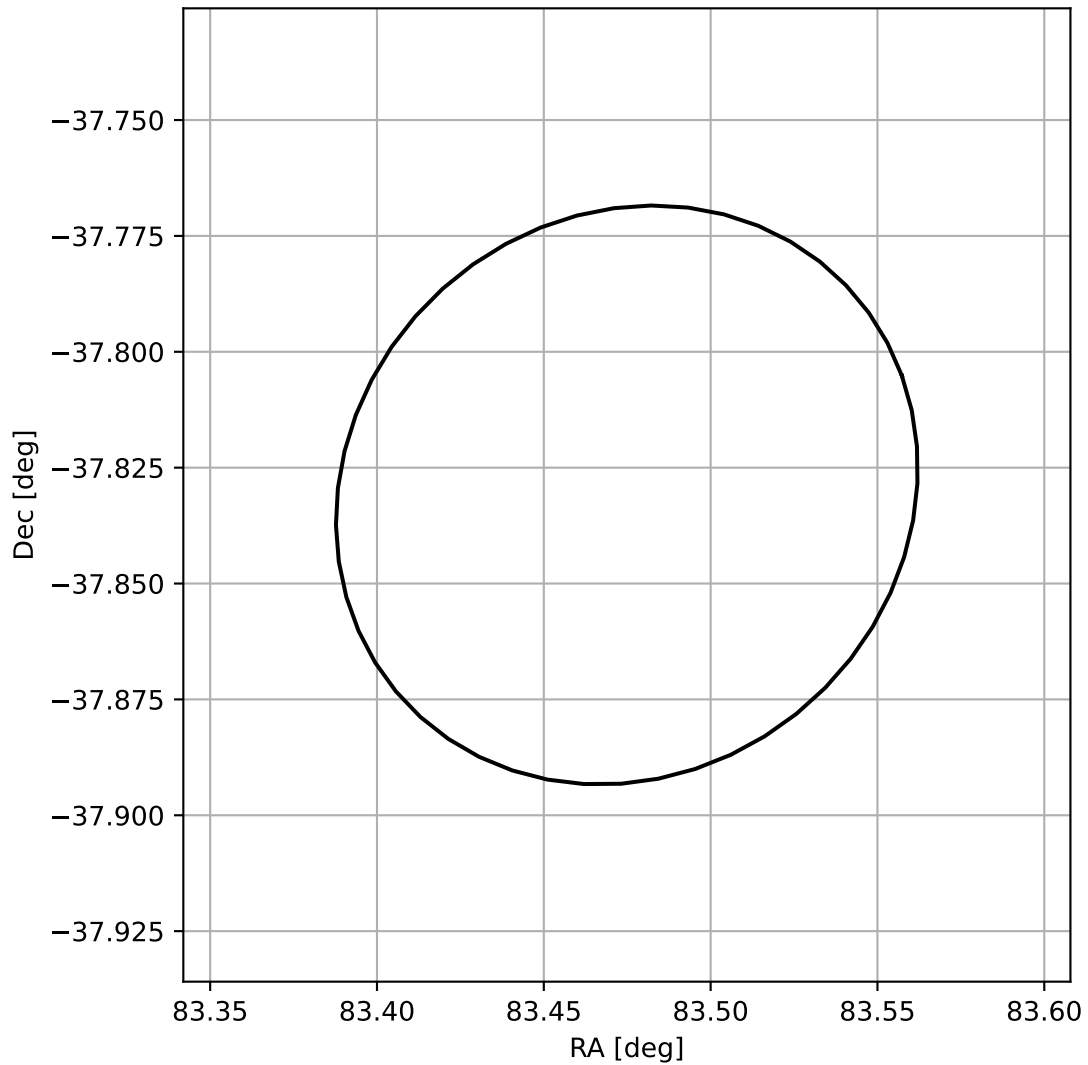
4FGL J0533.8-3749
