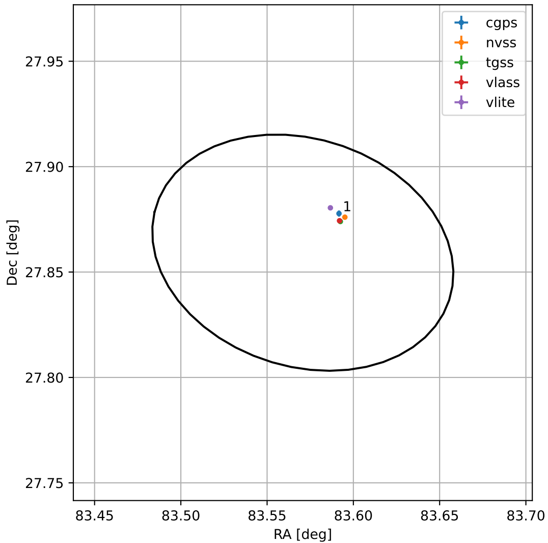
4FGL J0534.2+2751
