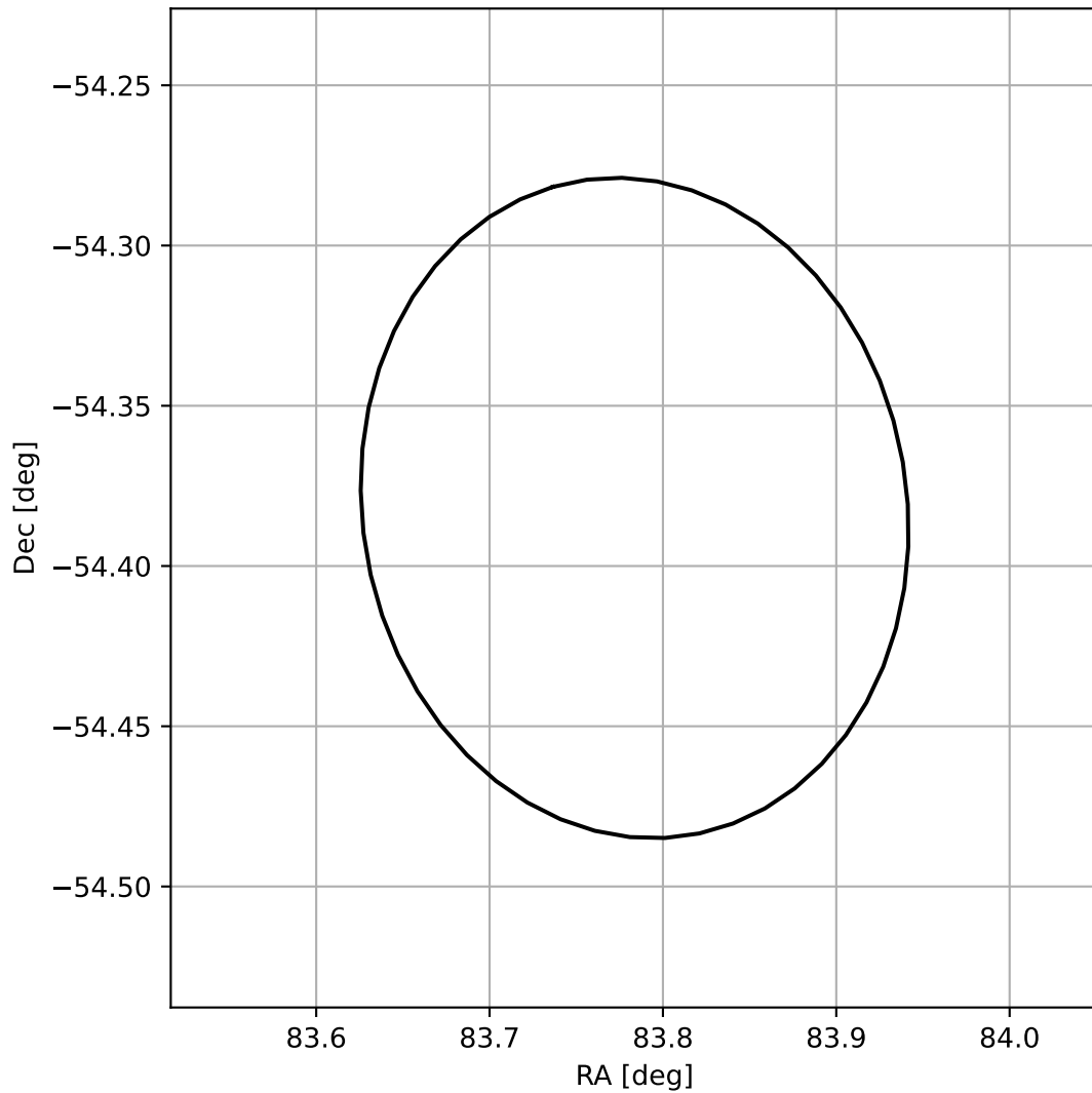
4FGL J0535.1-5422
