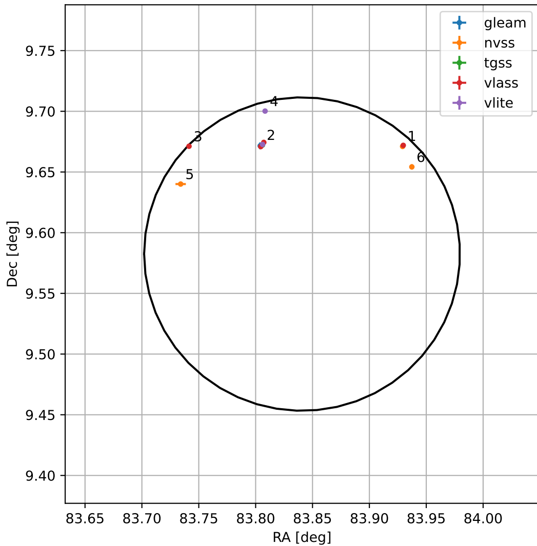
4FGL J0535.3+0934
