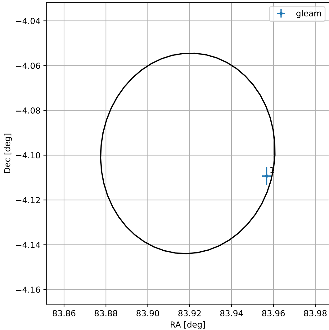
4FGL J0535.6-0405
