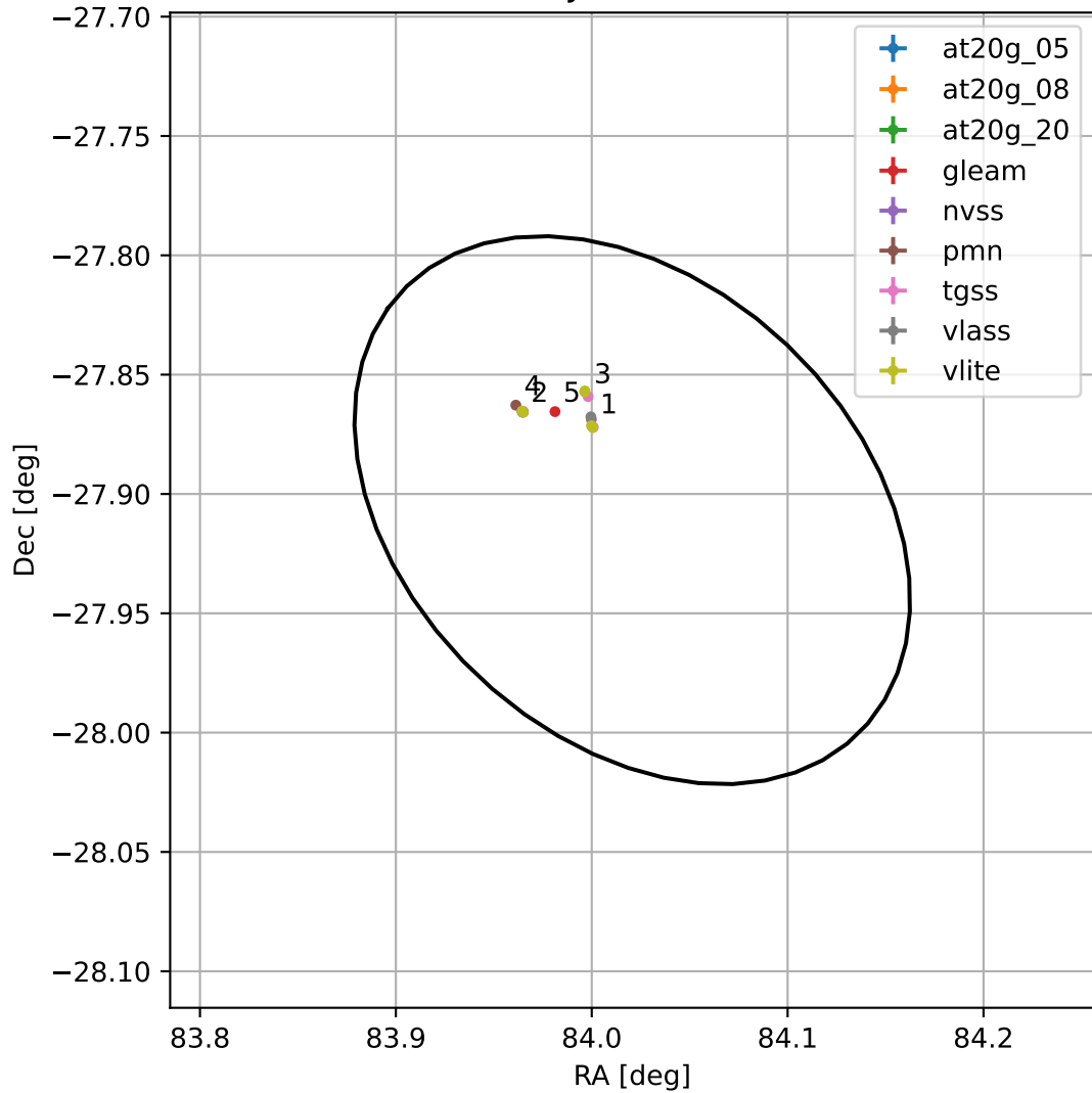
4FGL J0536.0-2754
