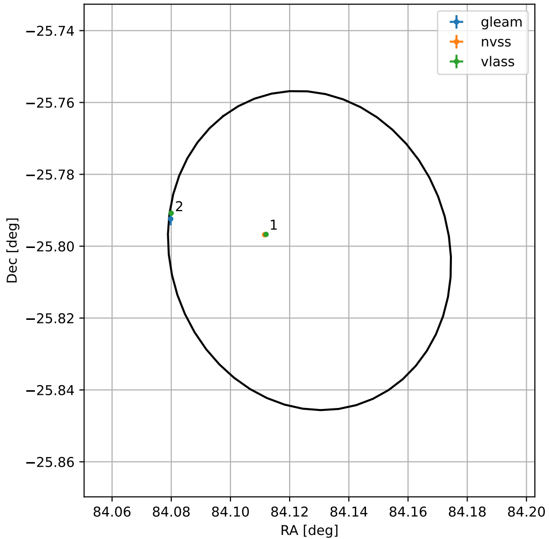
4FGL J0536.5-2548
