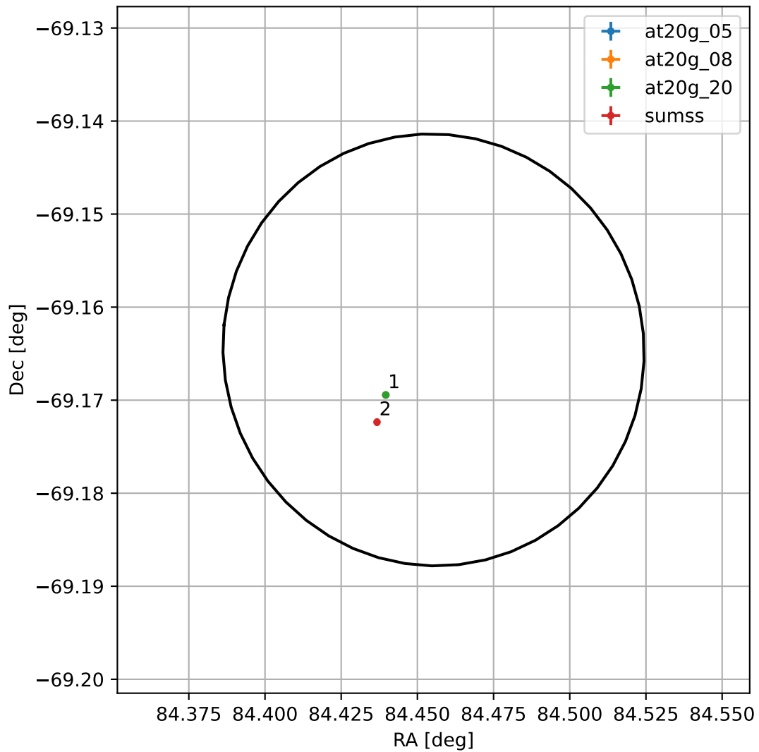
4FGL J0537.8-6909
