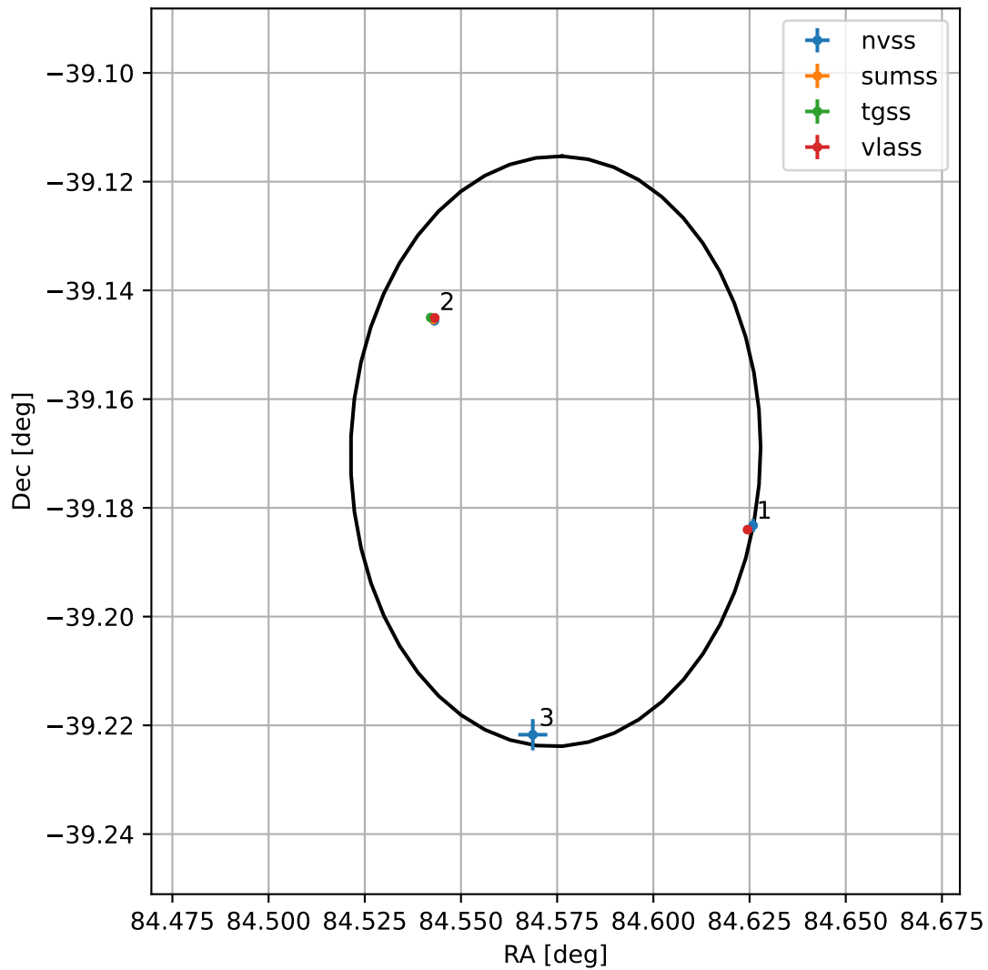
4FGL J0538.2-3910
