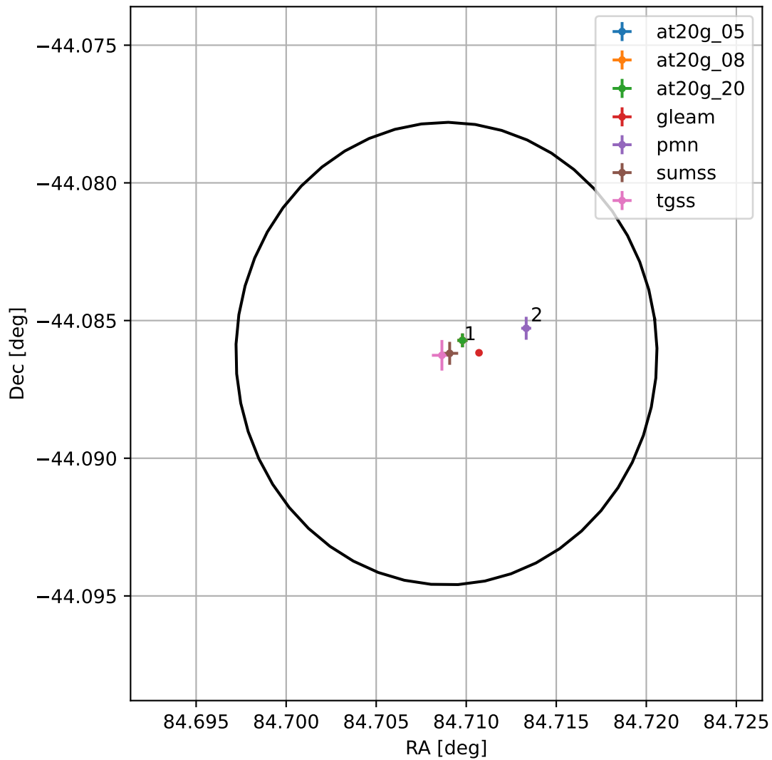
4FGL J0538.8-4405
