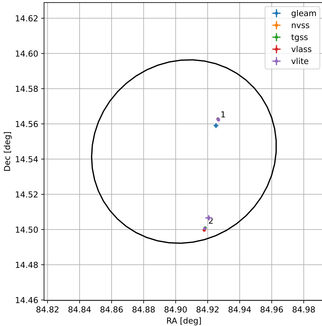
4FGL J0539.6+1432
