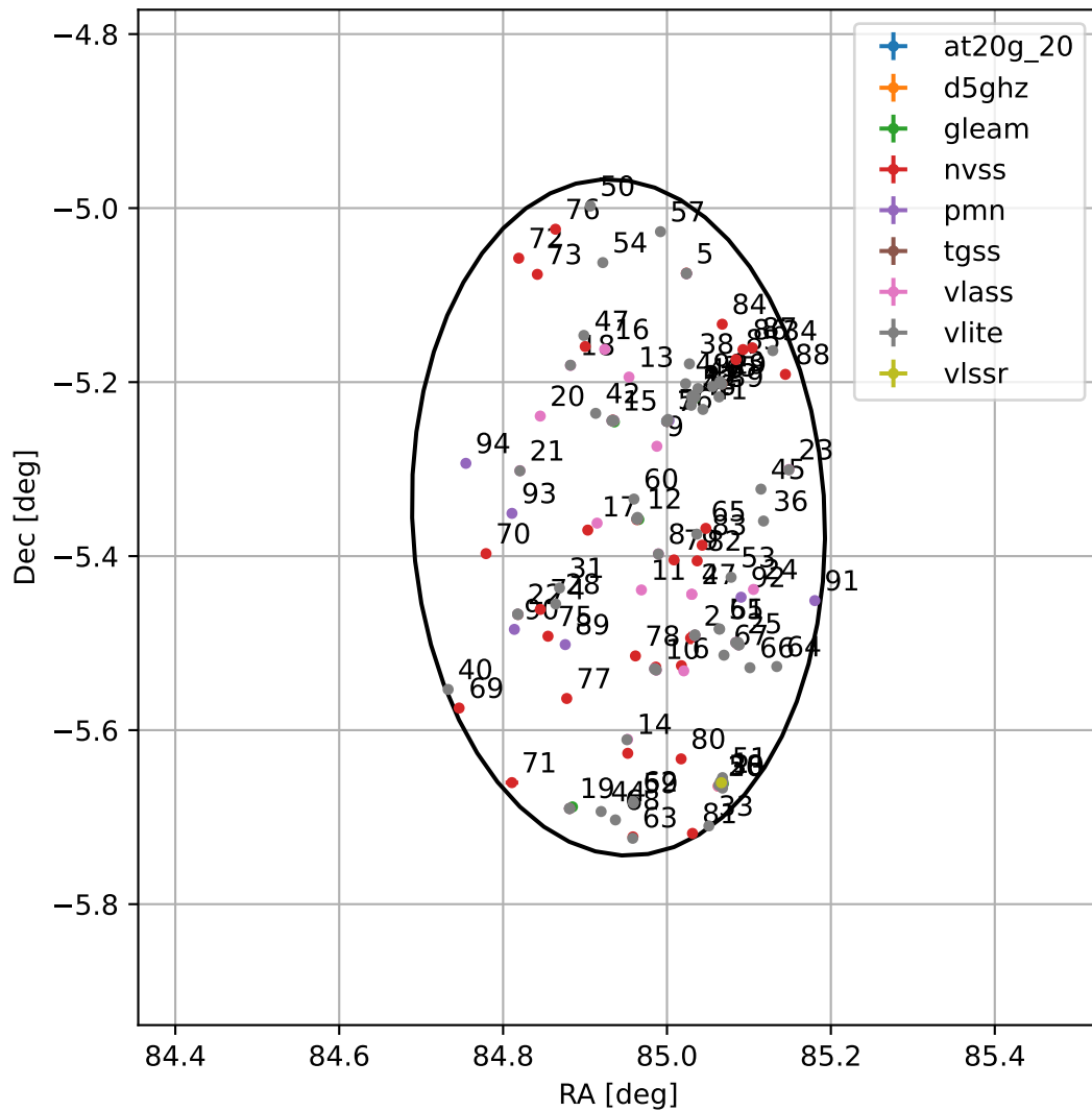
4FGL J0539.7-0521
