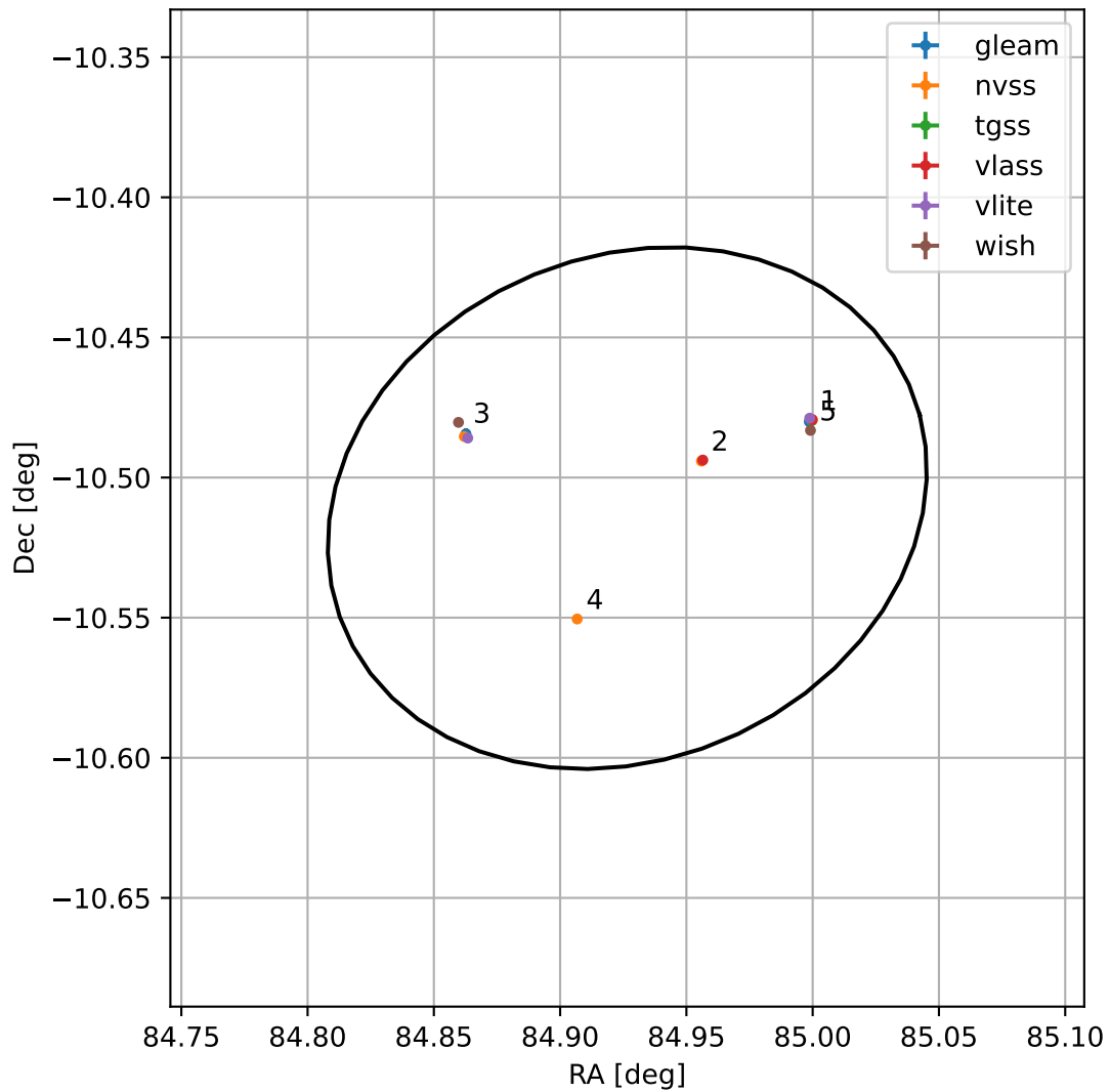
4FGL J0539.7-1030
