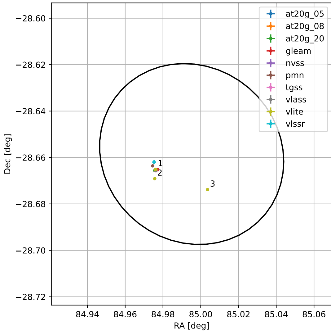
4FGL J0539.9-2839
