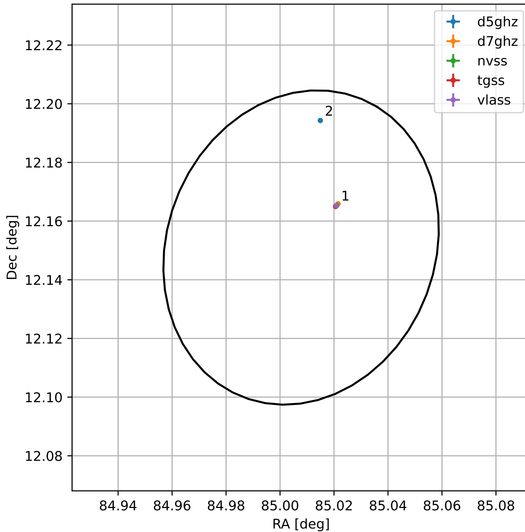
4FGL J0540.0+1209
