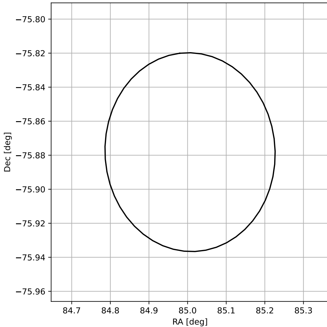
4FGL J0540.0-7552
