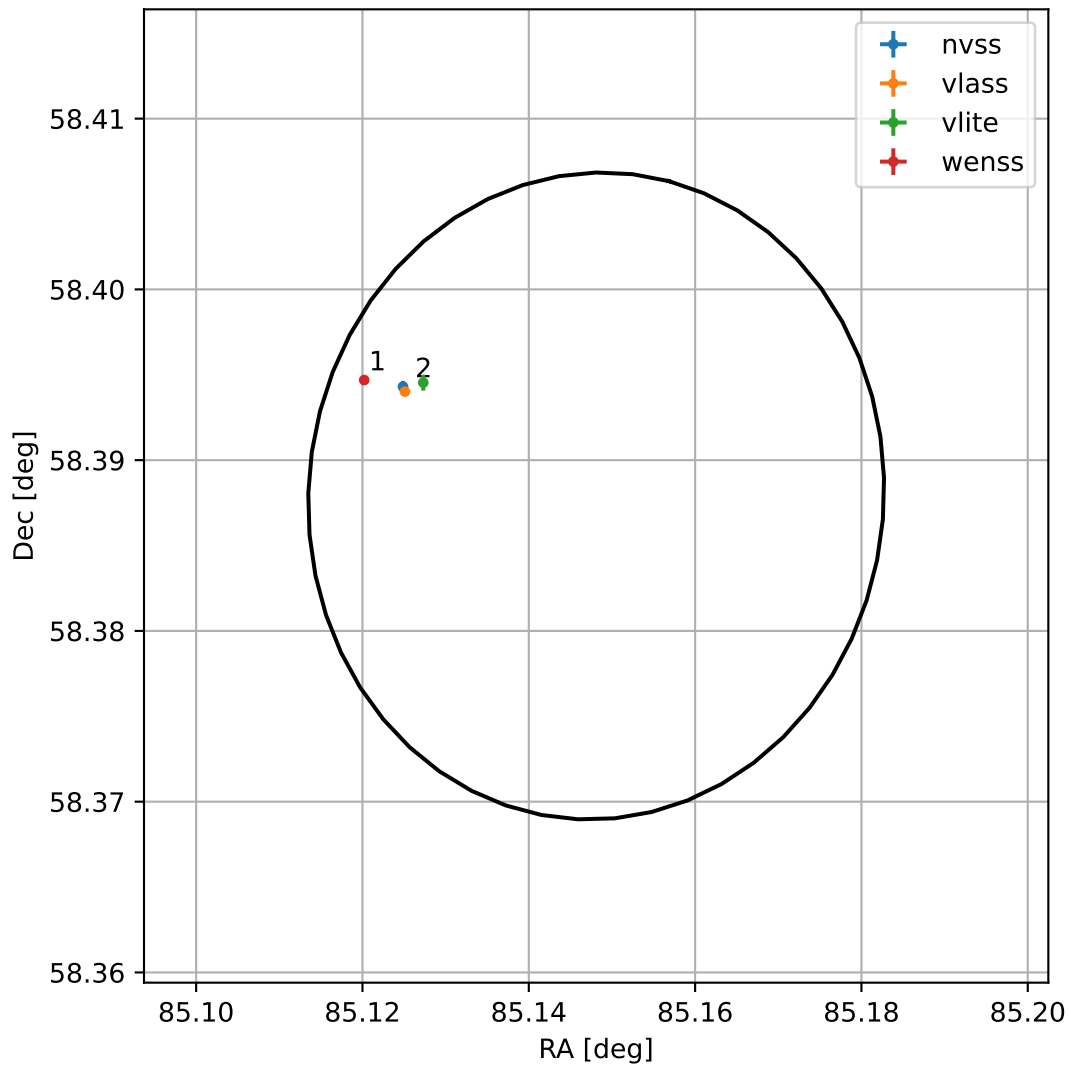
4FGL J0540.5+5823
