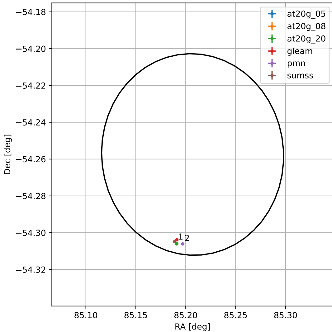
4FGL J0540.8-5415
