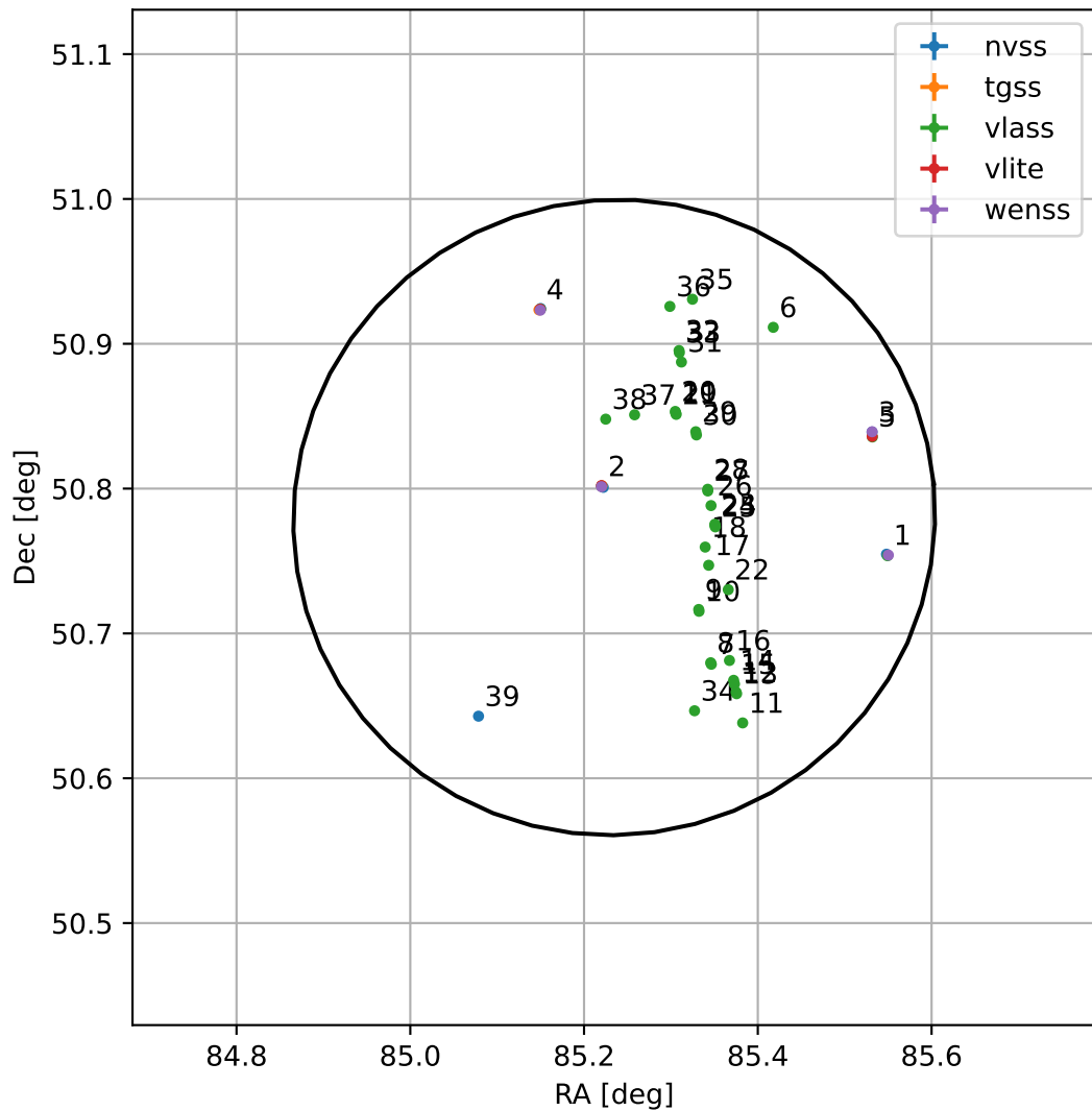
4FGL J0540.9+5046
