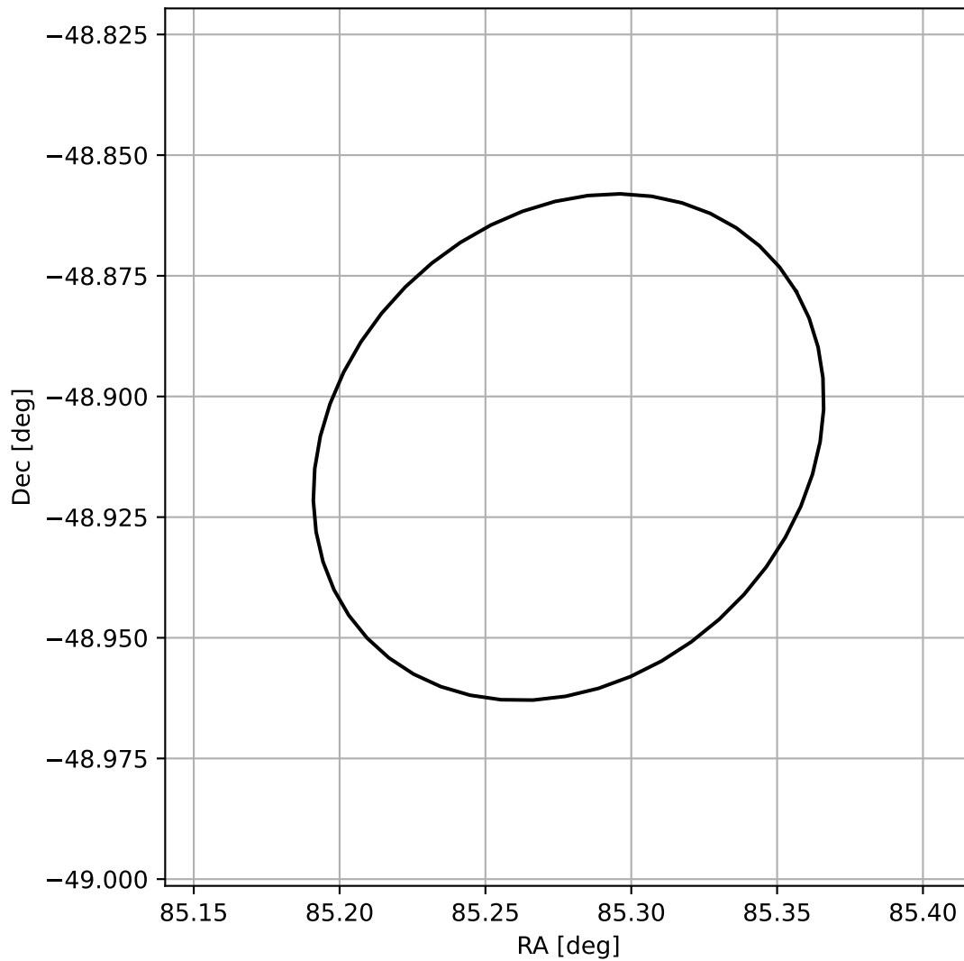
4FGL J0541.1-4854
