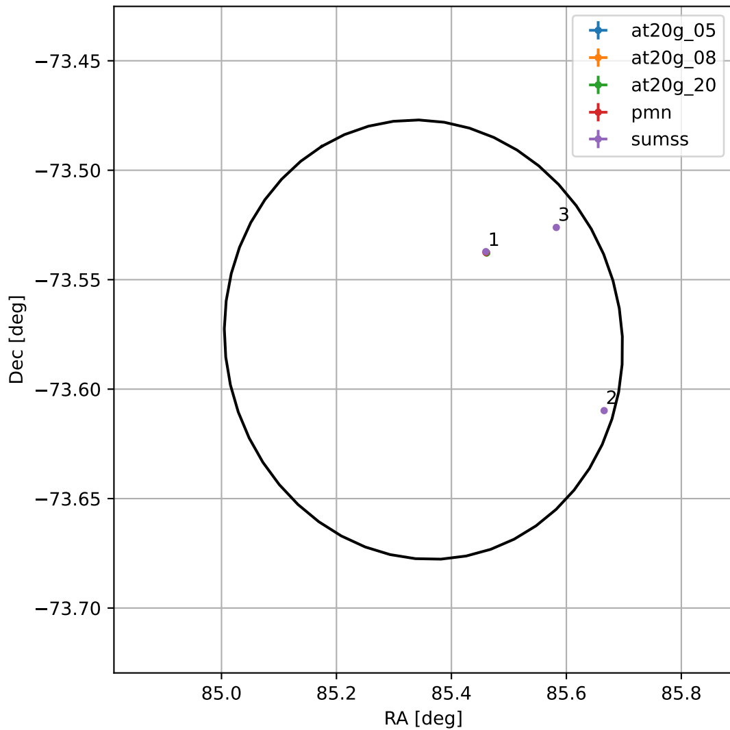
4FGL J0541.4-7334
