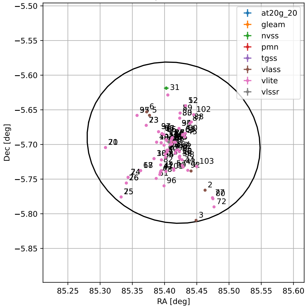
4FGL J0541.6-0541
