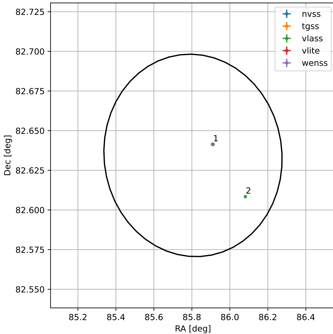
4FGL J0543.2+8238
